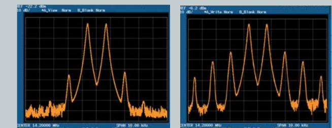
Class A: Ultra-Low TX IMD Class AB: Typical IMD at 200 W PEP Output
