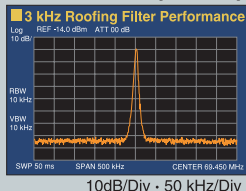
Three-section Roofing Filter Stage
