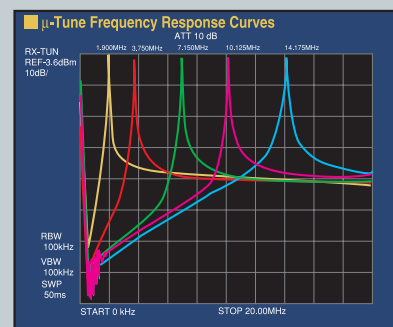
10dB/Div - 2 MHz/Div
